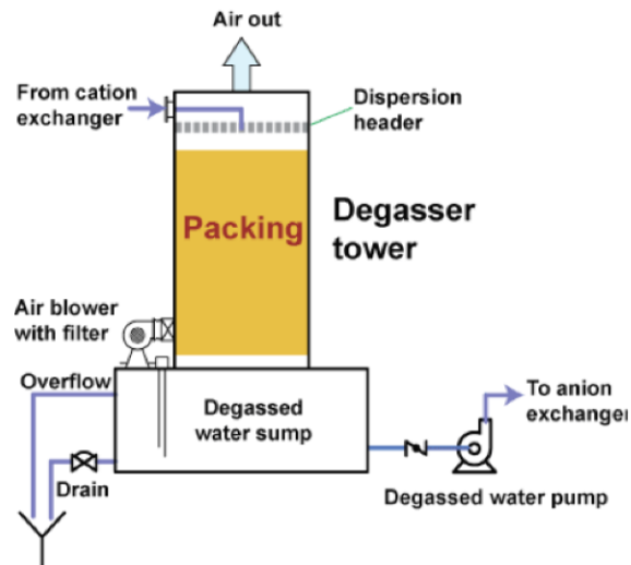
Degasser Towers
